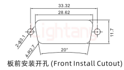
板前安装开孔 (Front Install Cutout)
