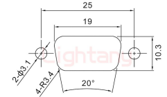
面板开孔 (Panel Cutout)
